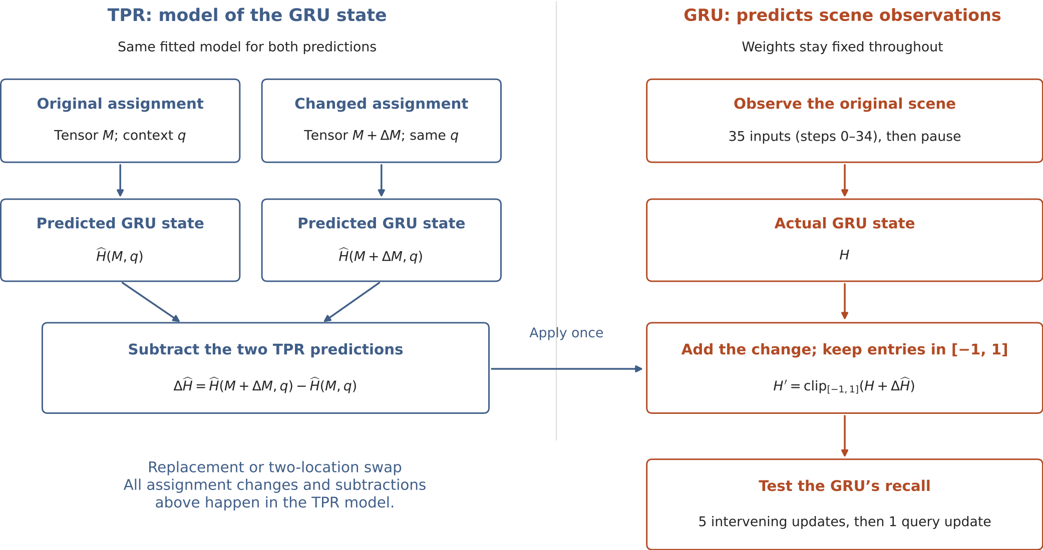
Figure 2. Calculate the edit in the TPR; test it in the GRU
