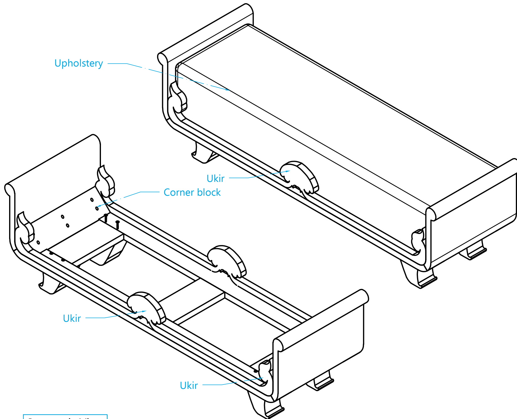
Isometric View
