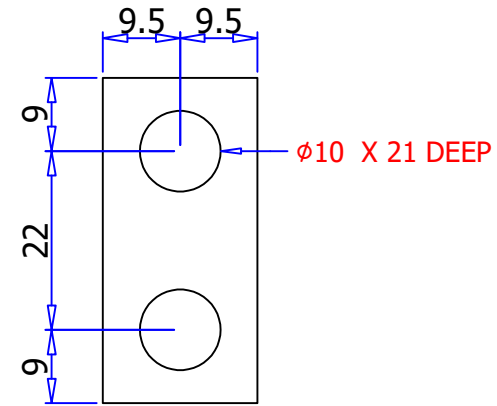
DETAIL U (1:1)
