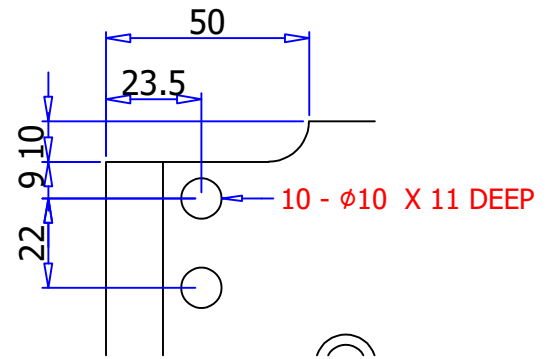
DETAIL F (1:2)
