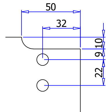
DETAIL H (1:2)
