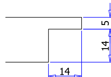
DETAIL D (1:1)
