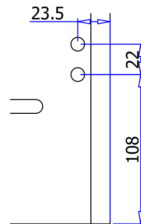
DETAIL C (1:3)
