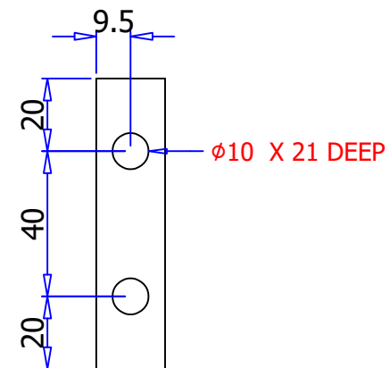
DETAIL T (1:2)
