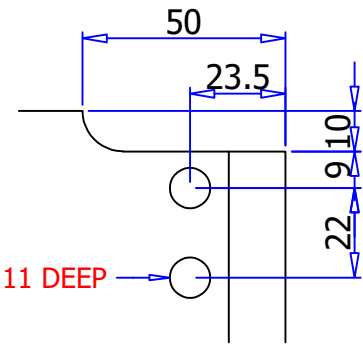
DETAIL B (1:2)
