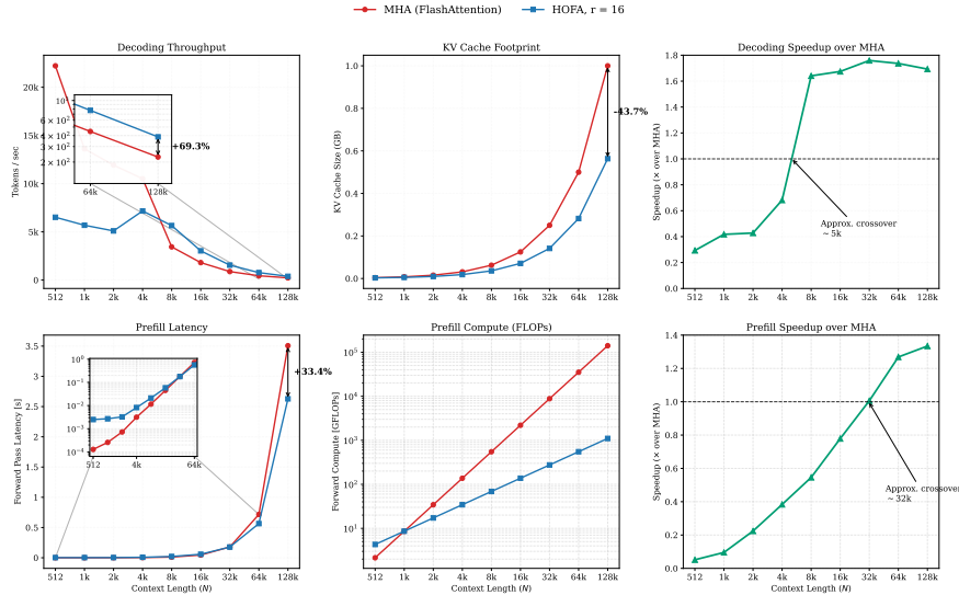
Figure 1: Hardware Execution & Throughput Benchmarks. Empirical autoregressive decoding throughput and KV-cache footprint scaling (top row) alongside prefill latency and compute scaling (bottom row) comparing HOFA to FlashAttention-2 MHA.
