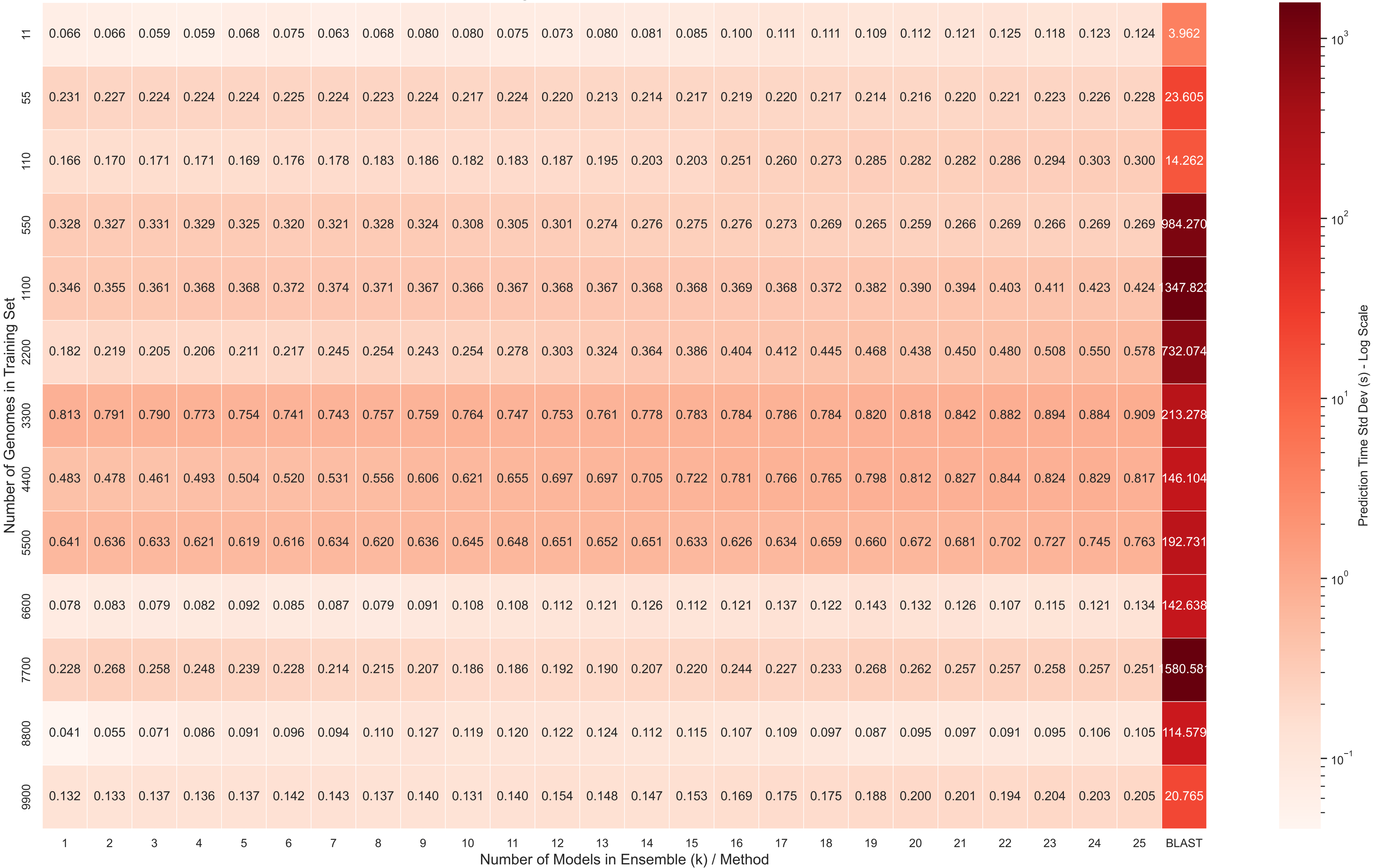
Time Stability Landscape: Ensemble vs. BLAST
