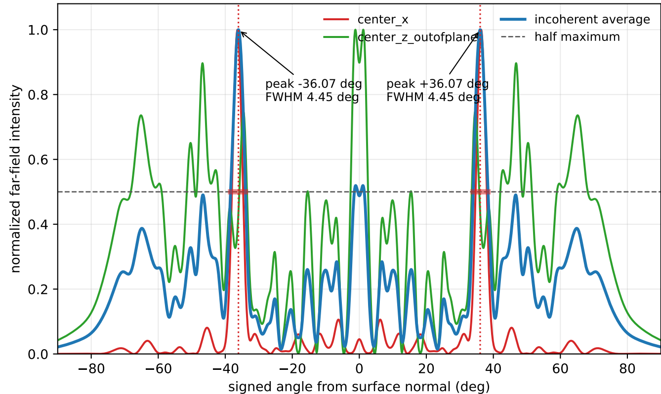
R2-2D 453 nm far-field angle cuts
