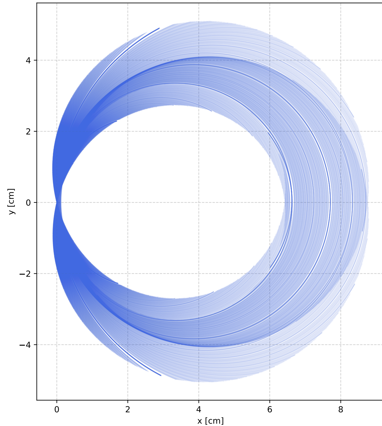
Reachable Workspace (Position)
