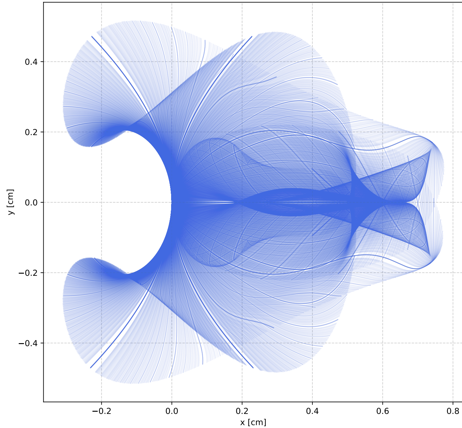
Reachable Workspace (Position)
