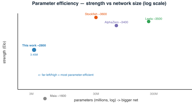
Figure 7: Parameter efficiency: strength vs. network size (log scale). This work is the far-left/high (most efficient) point.
