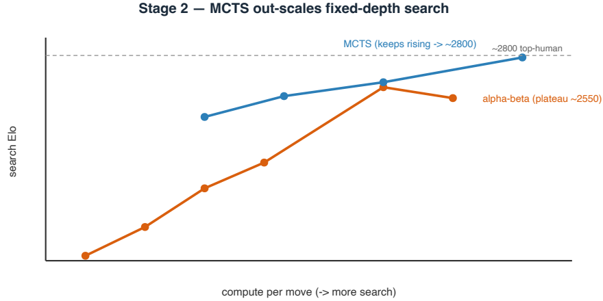
Figure 2: Stage 2: MCTS beats and out-scales fixed-depth search.
