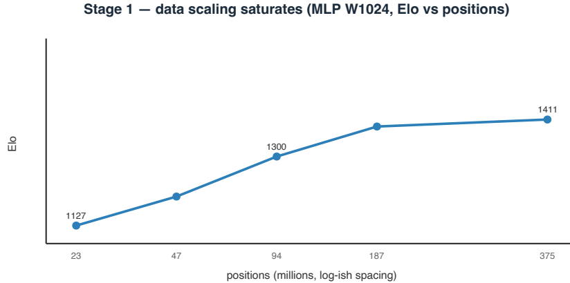
Figure 1: Stage 1: single-pass strength saturates with data (MLP W1024).
