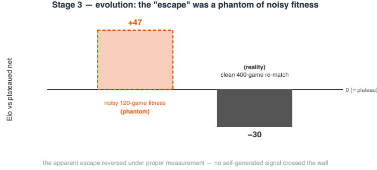
Figure 6: Stage 3: the evolution “escape” was a phantom—noisy fitness said +47 Elo, a clean re-match said −30.
