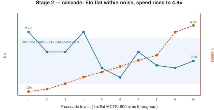
Figure 3: Stage 2: the wide→narrow cascade holds Elo (within noise) while cutting per-move compute up to 4.8x.
