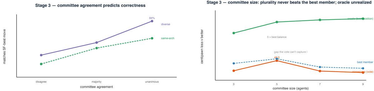
Figure 5: Left: committee agreement predicts correctness (robust). Right: plurality voting never beats the best member, and adding correlated members reverts the gain.
