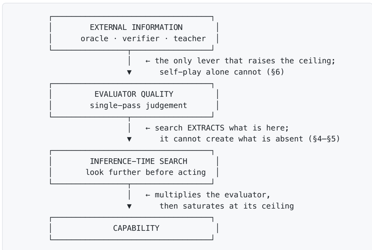
Figure 1 — one causal chain, four instantiations. The whole paper is a single chain: external information is the only lever that raises evaluator quality ; inference-time search extracts — never creates — what the evaluator already contains; the two compose into capability (strength = evaluator \times search). Each arrow carries a load-bearing result of this work.
