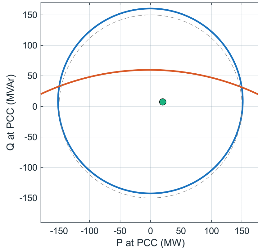
Filtered test: G_f=0.002 , B_f=0.0887
