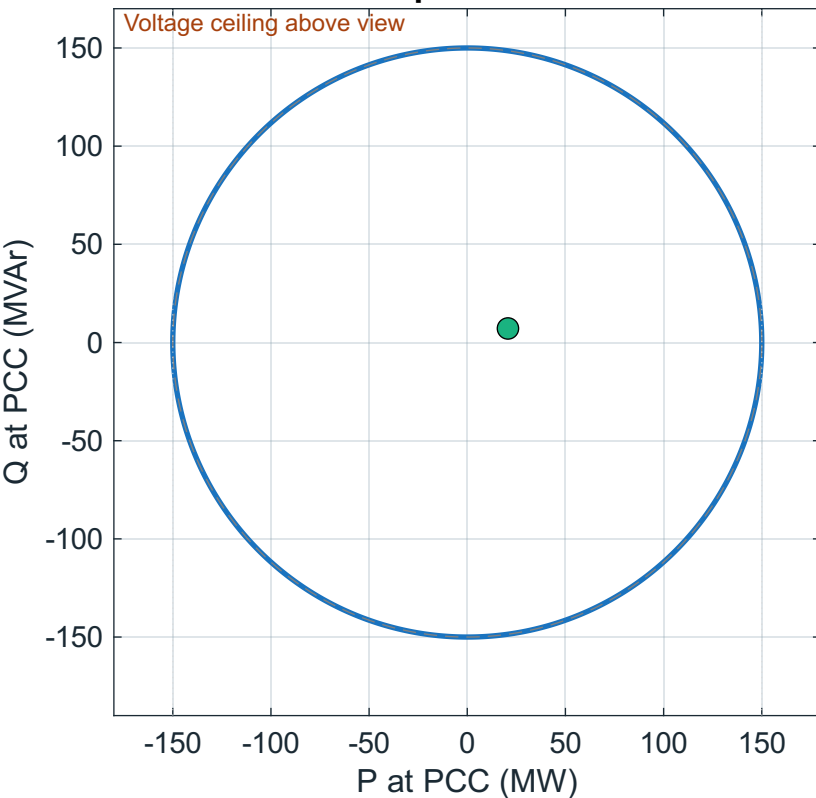
Five-bus replication: no filter
