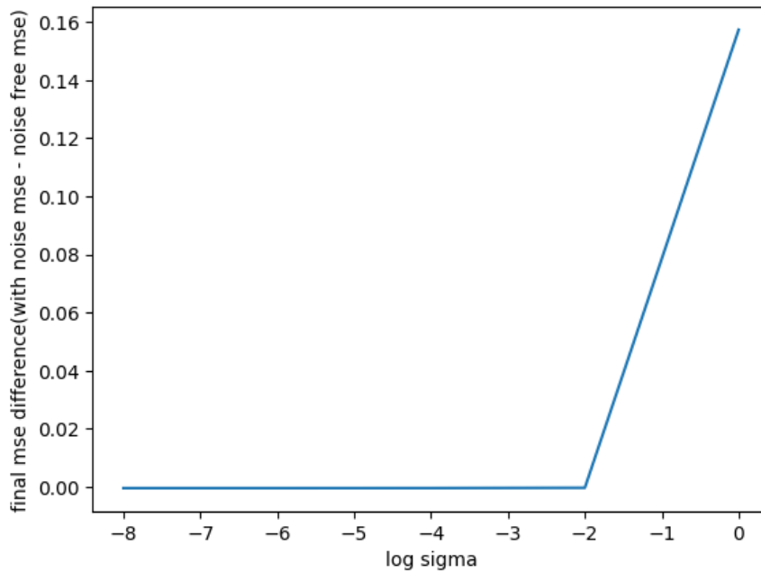
method COBYLA - final mse difference(with noise mse - noise free mse) over log sigma
