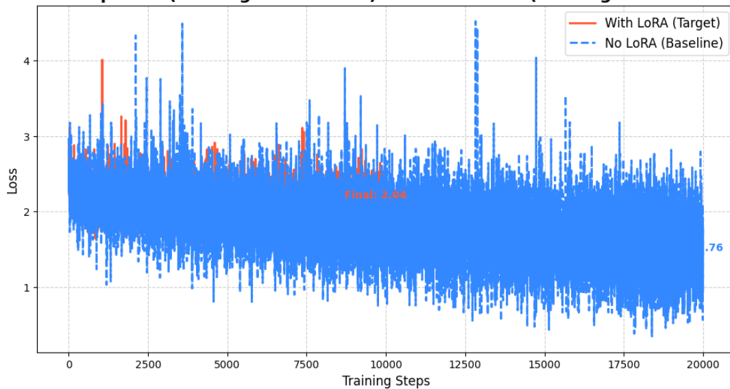
LoRA Adaptation(training time 7246.9) vs Baseline FFT(training time 10918.14)
