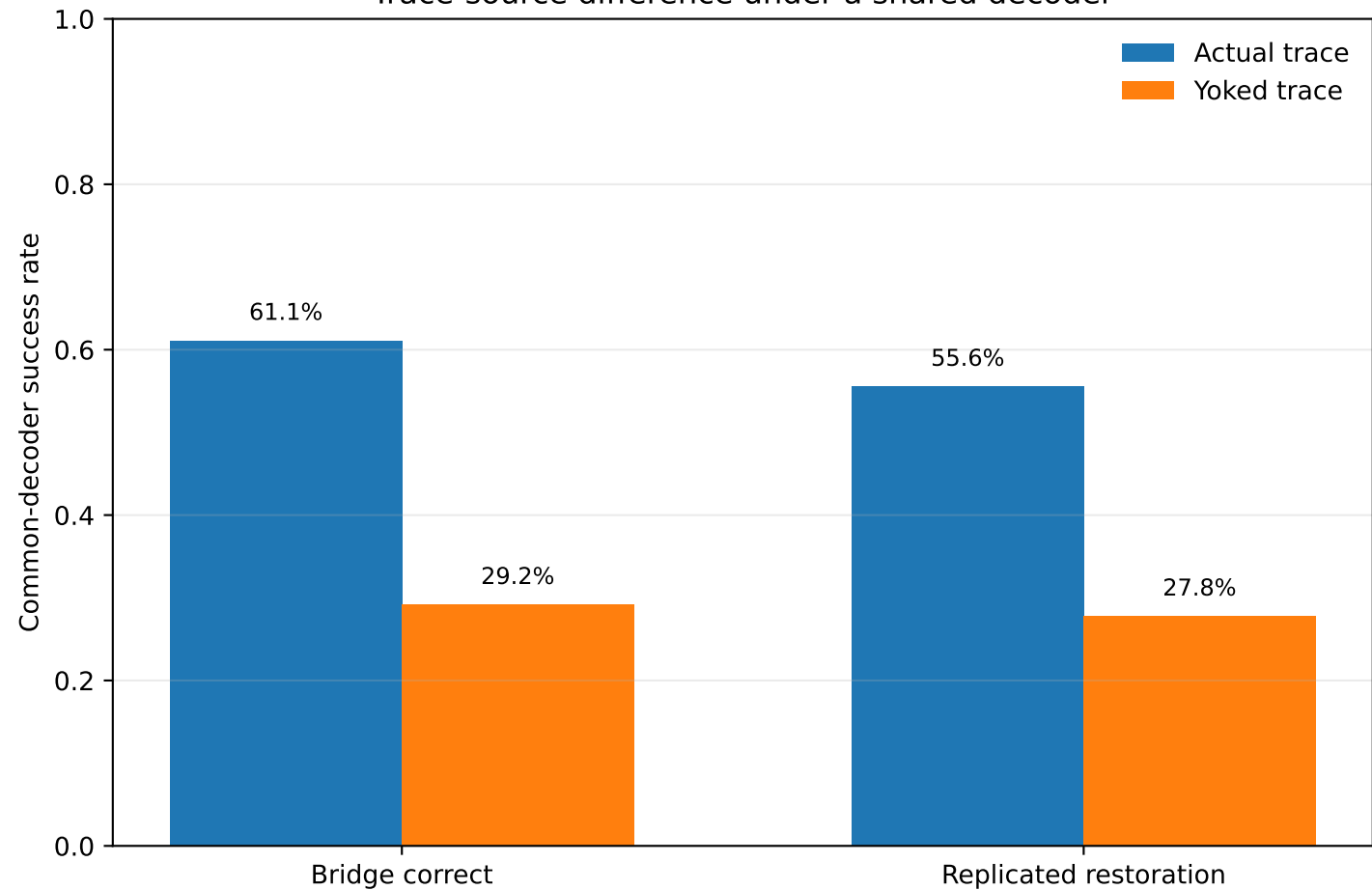
Trace-source difference under a shared decoder
