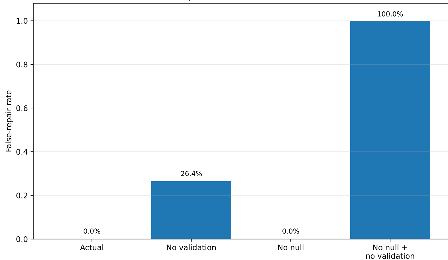
Safety ablations in neutral worlds
