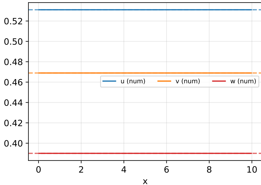
(b) final field vs analytic (dashed)
