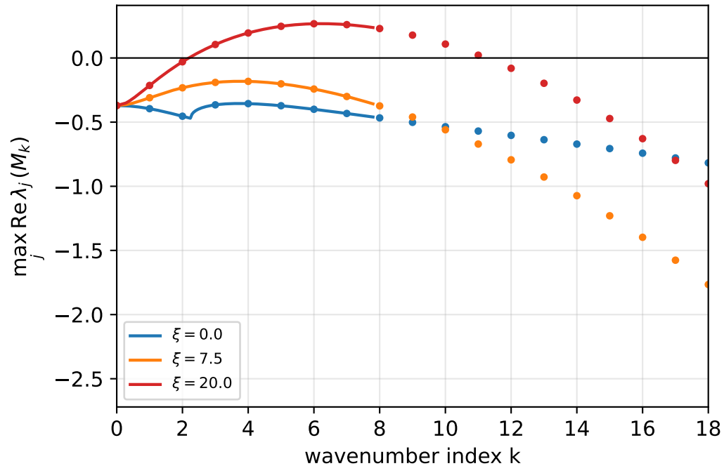
(a) dispersion relation
