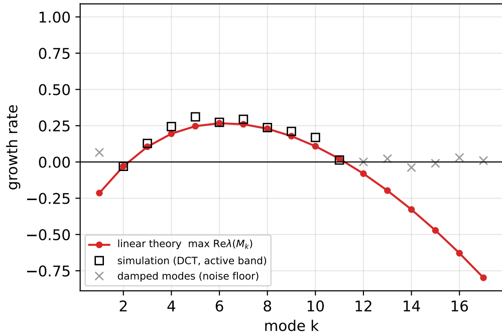
(b) modal growth rates, \xi = 20.0
