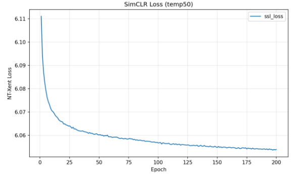
Figure 4b: Loss ( \tau=5.0 )
