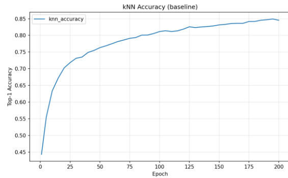
Figure 1b: kNN Accuracy ( k=20 )
