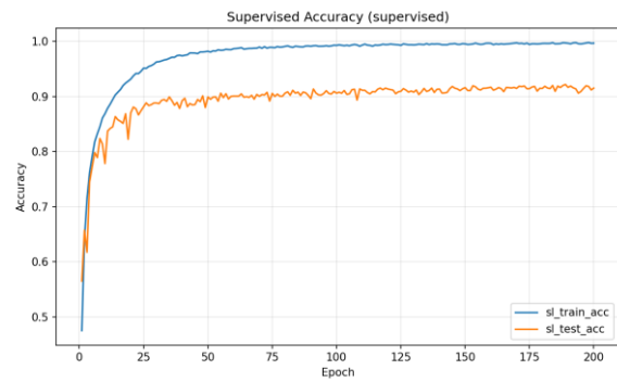
Figure 3b: Supervised Accuracy
