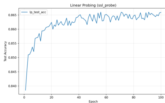
Figure 2: SSL Linear Probing Accuracy on CIFAR-10
