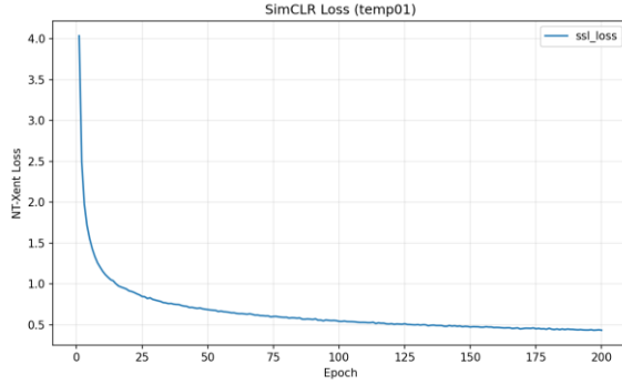
Figure 4a: Loss ( \tau=0.1 )
