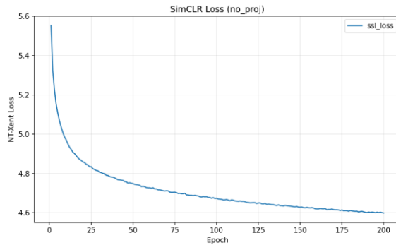
Figure 6a: No Projector — Loss
