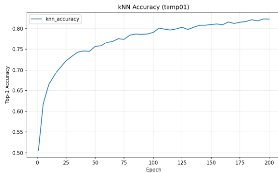
Figure 5a: kNN ( \tau=0.1 )
