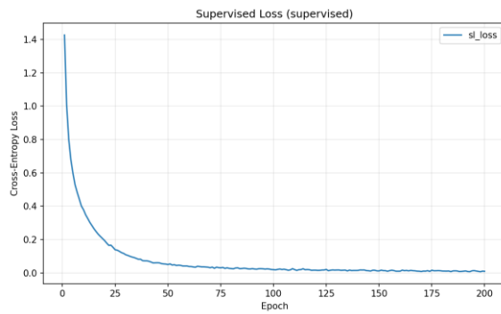
Figure 3a: Supervised Loss
