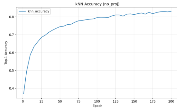
Figure 6b: No Projector — kNN
