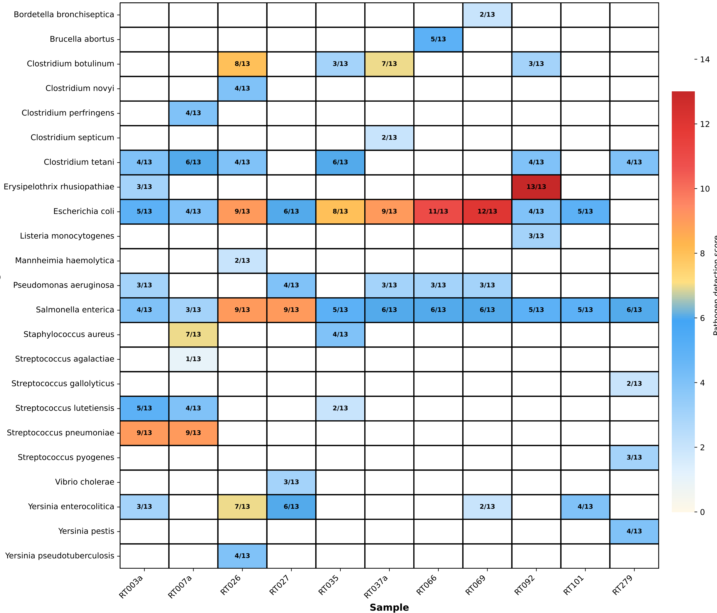
Pathogen Detection Scores Across All Samples
