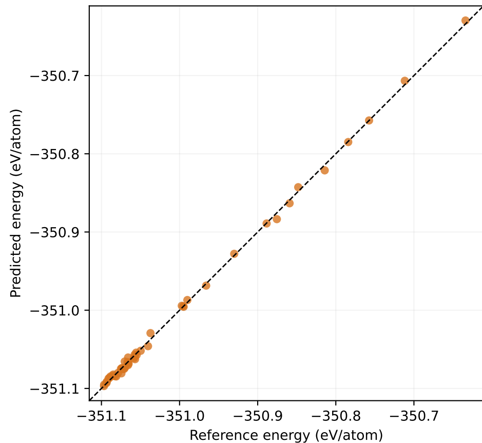
03 · Equal weights / learned offset: energy MAE 2.821, RMSE 3.503 meV/atom
