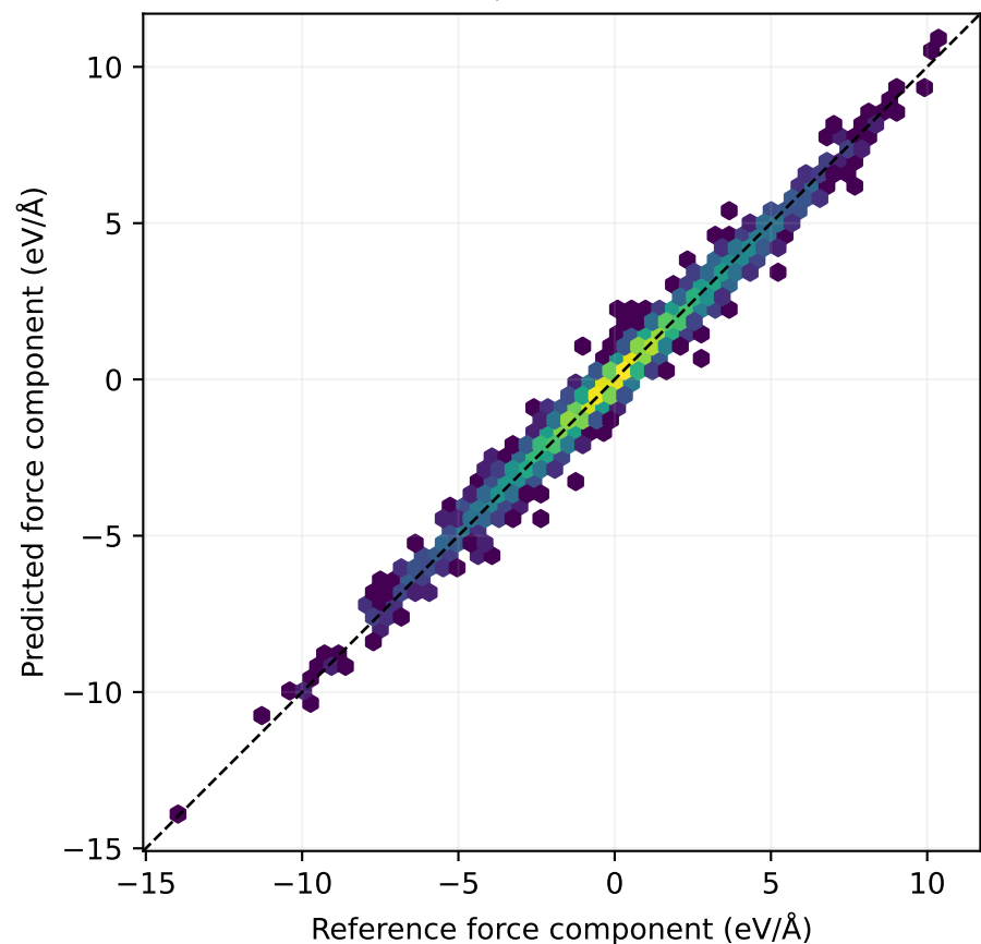
03 · Equal weights / learned offset: forces MAE 0.1209, RMSE 0.1798 eV/Å
