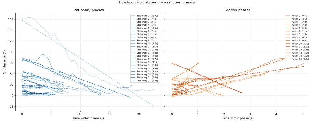
Figure 5: Trial for h=0.2 non adaptive. Stationary phases is a period of time over .5 seconds where the angular velocity stayed under 0.15 rad/s during that time. A motion phase is equivalent except velocity must stay above 0.15 rad/s
