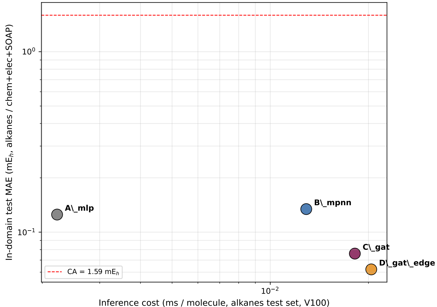
Accuracy vs. inference cost per architecture (alkanes)
