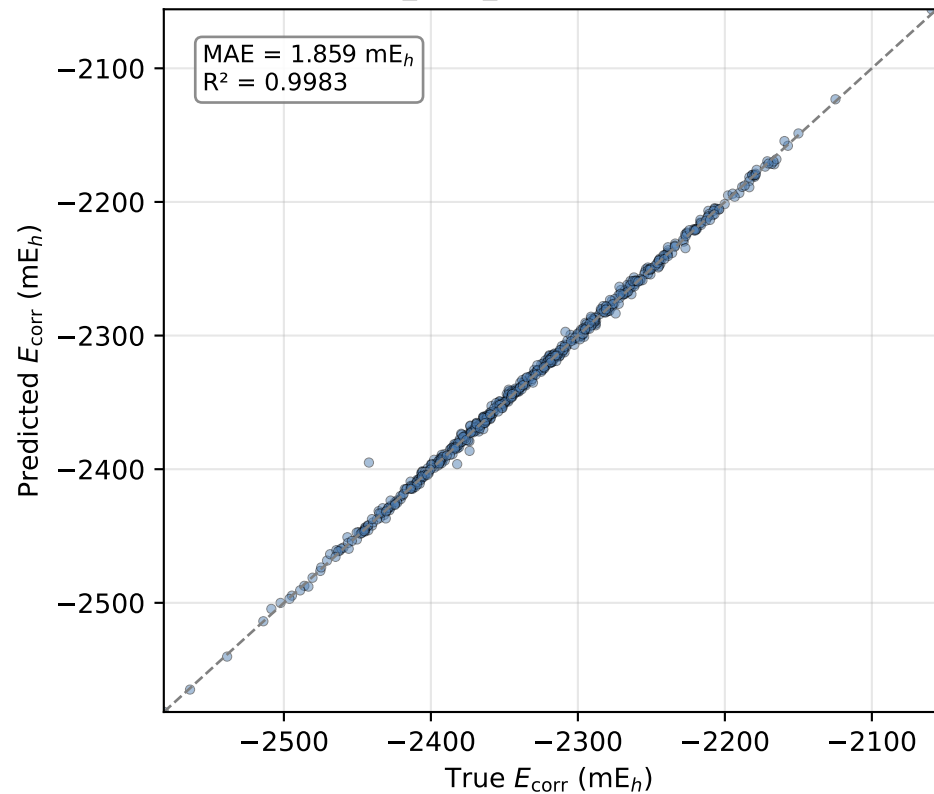
GDB-13-T (D\gat\_edge / chem+elec+SOAP)
