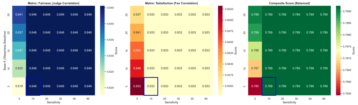
Figure 17: Parameter Sensitivity Analysis for the Adaptive System
