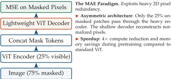
SSL VISION PARADIGMS COMPARISON
