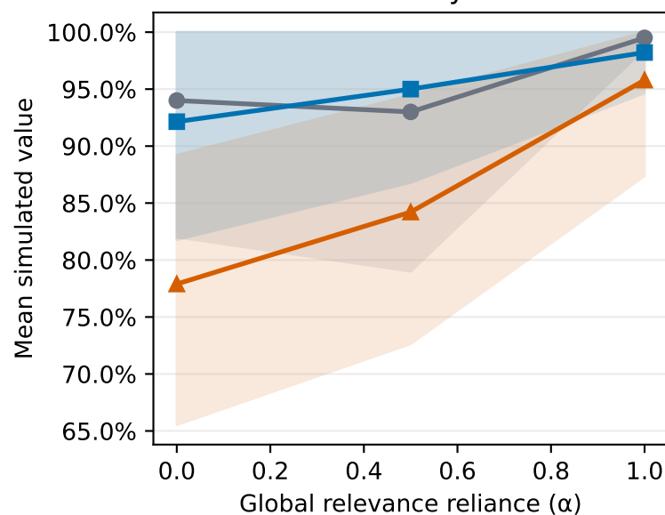
Actionability rate
