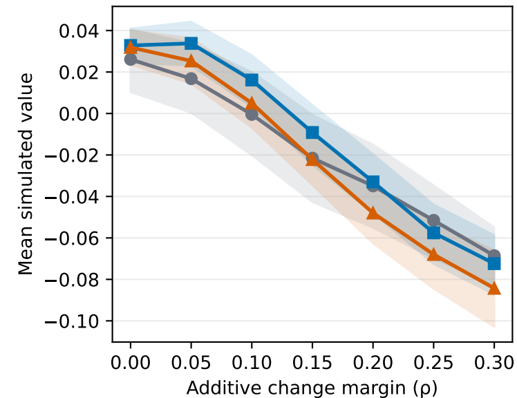
Boundary-distance improvement
