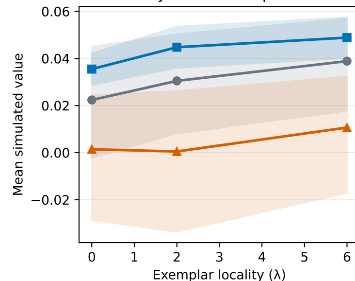
Boundary-distance improvement
