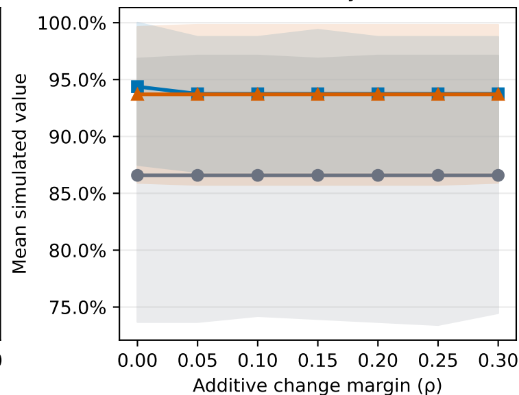
Actionability rate
