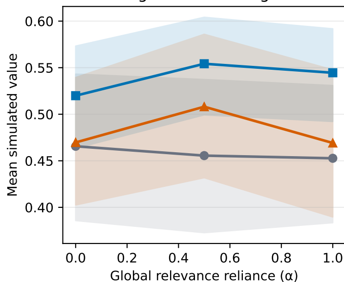
Target-confidence gain
