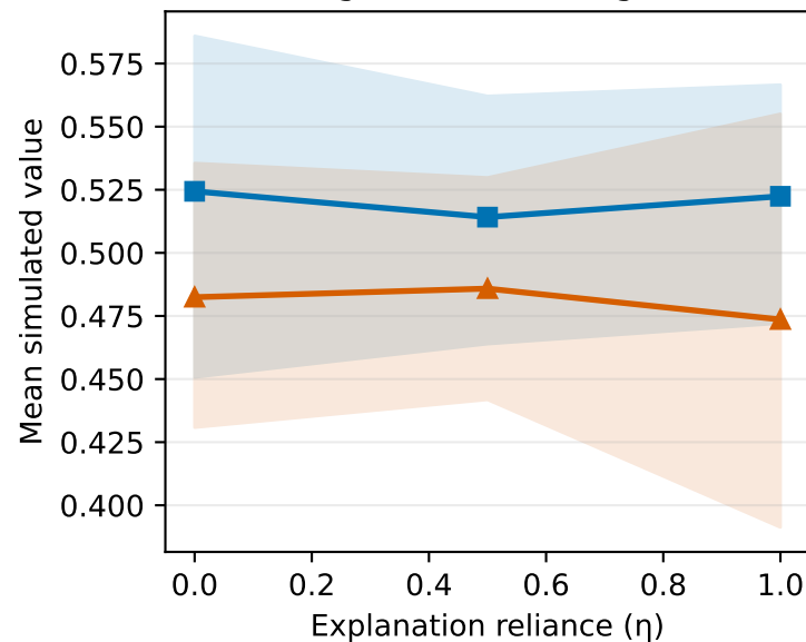
Target-confidence gain
