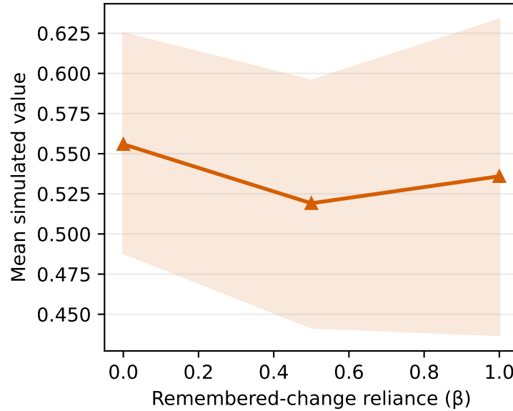
Target-confidence gain
