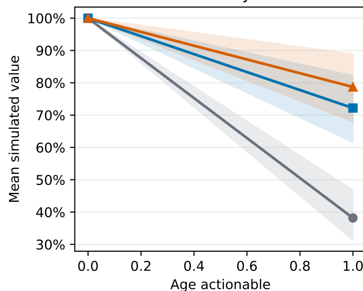
Actionability rate
