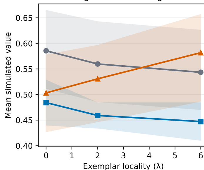
Target-confidence gain
