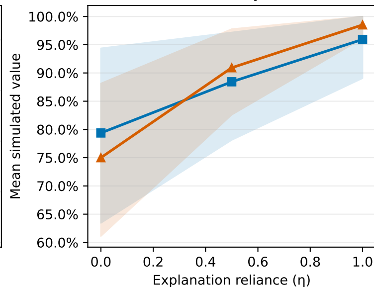
Actionability rate
