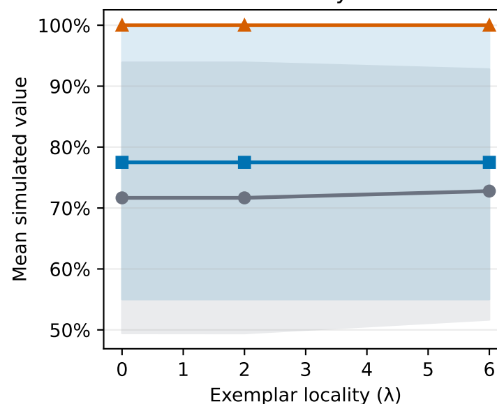
Actionability rate
