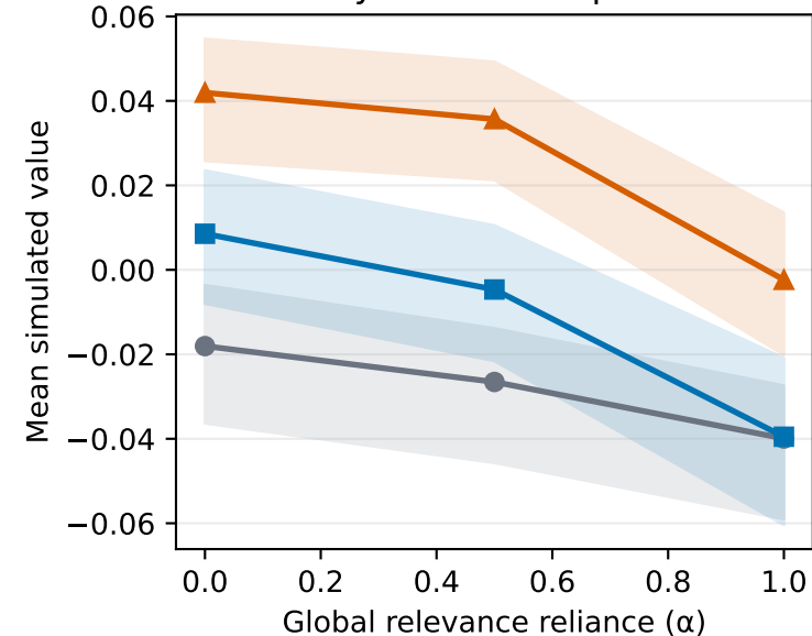
Boundary-distance improvement
