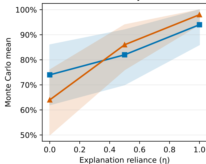
Actionability rate
