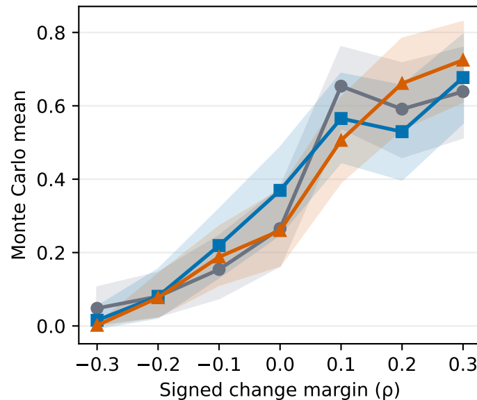
Target-confidence gain
