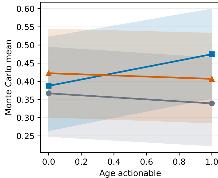
Target-confidence gain
