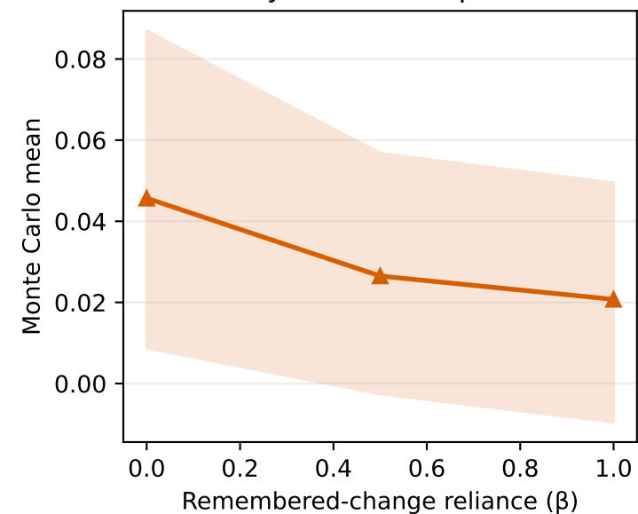
Boundary-distance improvement
