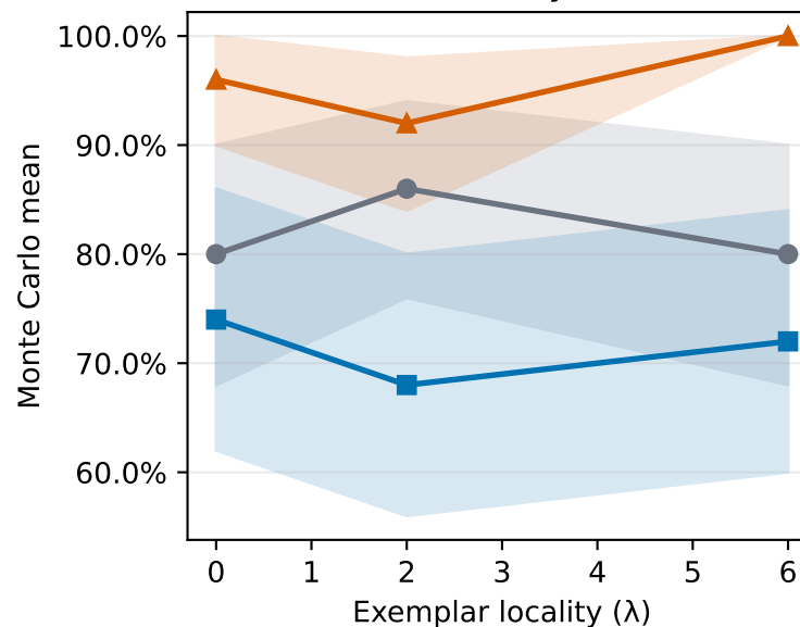
Actionability rate
