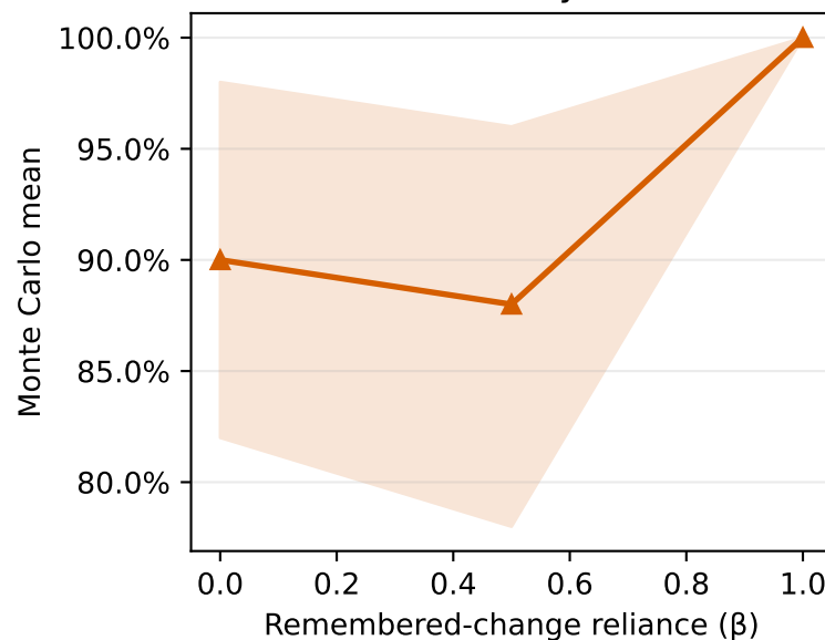
Actionability rate
