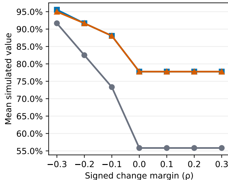
Actionability rate
