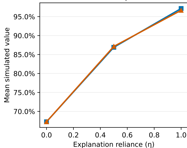
Actionability rate
