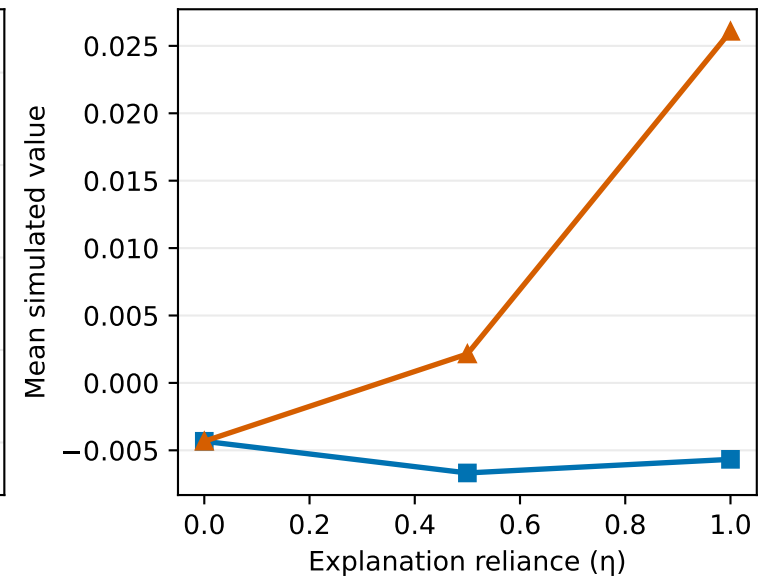
Boundary-distance improvement
