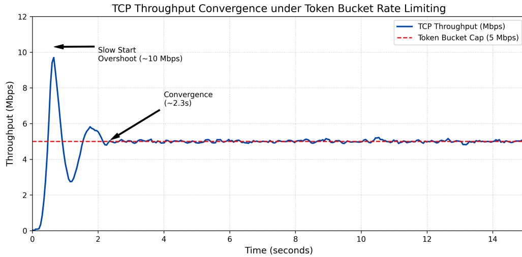
Figure 6.1: Throughput graph showing TCP CUBIC converging from an initial 10 Mbps burst to the 5 Mbps Token Bucket cap over approximately 2.3 seconds.
