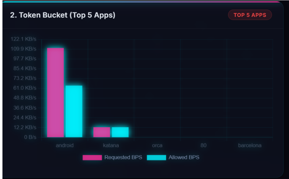
Figure 5.1: Token Bucket enforcement in action: aggressive throttling of low-priority background processes versus full allocation for foreground apps.
