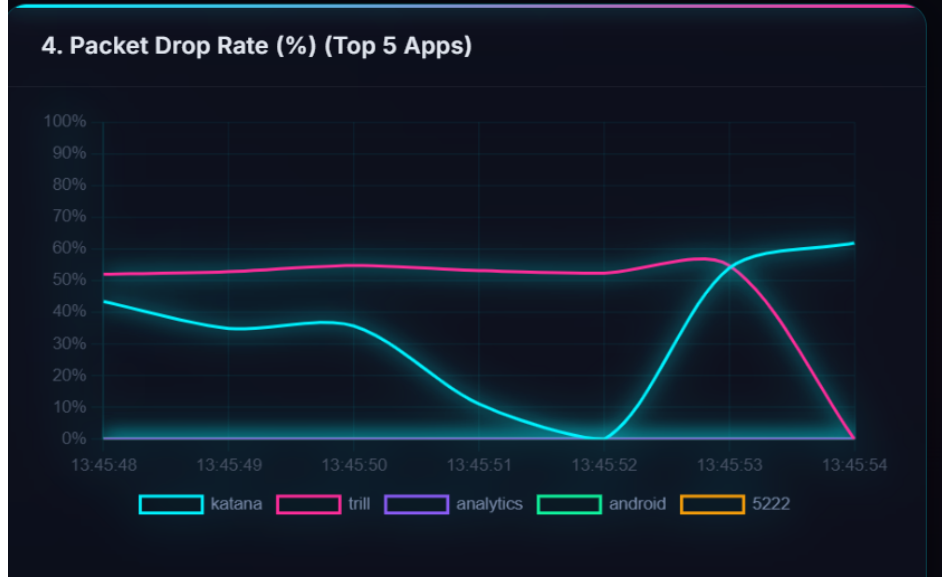
Figure 5.3: Packet Drop Rate dynamics during network congestion. The X-shape cross-over demonstrates Token Bucket effectively suppressing greedy flows to relieve Bufferbloat.
