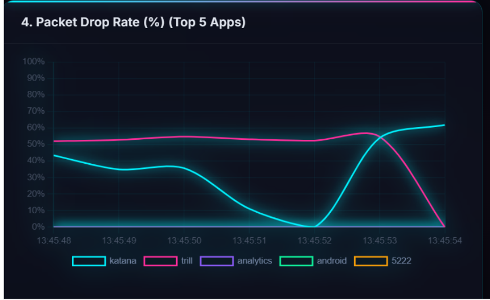
Figure 6.3: Packet Drop Rate dynamics during bandwidth contention. The characteristic X-shaped cross-over between trill (TikTok, ~50%) and katana (Facebook, ~60%) demonstrates the Token Bucket dynamically suppressing greedy flows. As TCP/QUIC congestion control reacts to packet drops, the suppressed flow reduces its rate, causing the competing flow to increase—and subsequently be throttled in turn.
