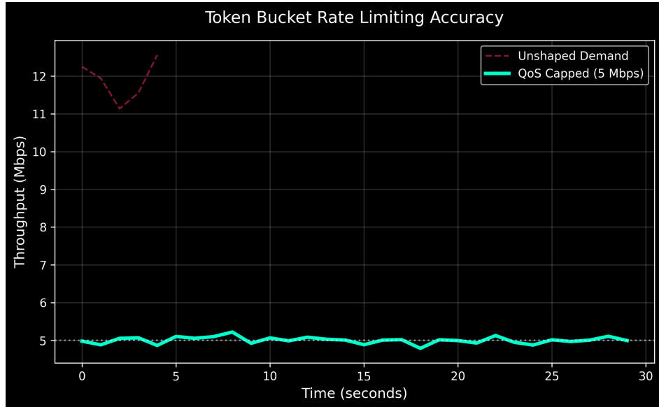
Figure 5.1: TCP throughput convergence to the 5 Mbps cap.
