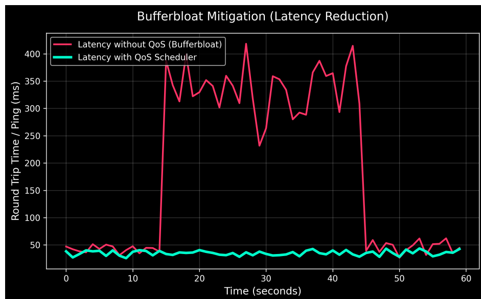
Figure 5.3: Latency comparison: baseline Bufferbloat vs. QoS-enabled.
