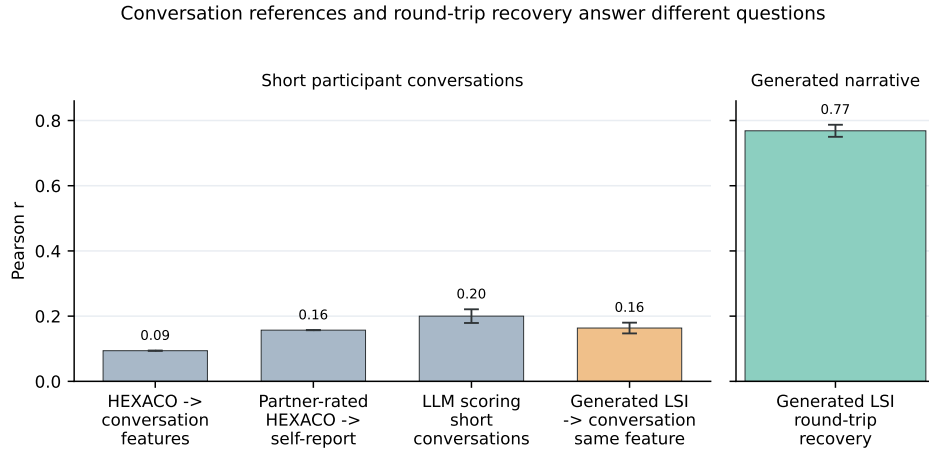
Figure 3: Short PARSEL conversations provide a low-bandwidth participant-language reference. The left panel shows participant-language references derived from short conversations; the right panel shows generated-LSI round-trip recovery, a different construct measured from the full generated narrative.
