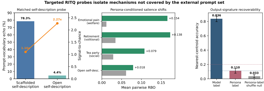
Figure 3: The RITQ diagnostic bank isolates mechanism-level contrasts. Left: removing phenomenological cue words from a matched self-description prompt sharply lowers prompt-vocabulary echo while increasing signal-to-chance. Middle: grey bars report unconditioned cross-model RBO and green bars report same-persona cross-model RBO for four targeted questions; persona-conditioned salience shifts are largest on the emotional-pain, retirement, and tea-party probes and smallest on the open self-description probe. Right: model identity is strongly recoverable from targeted-probe output signatures, while persona identity is weak but above a model-preserving shuffle null. Dotted lines mark naive chance levels.
