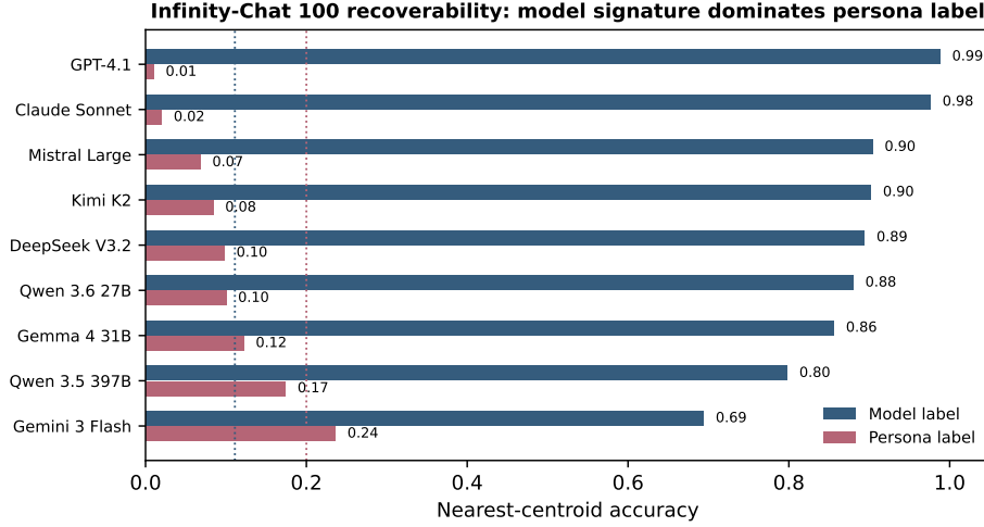
Figure 2: Nearest-centroid recoverability on Infinity-Chat 100 conditioned cells. Across models, the full output signature is far more recoverable by base model than by persona label. Dotted lines mark naive model and persona chance levels.
