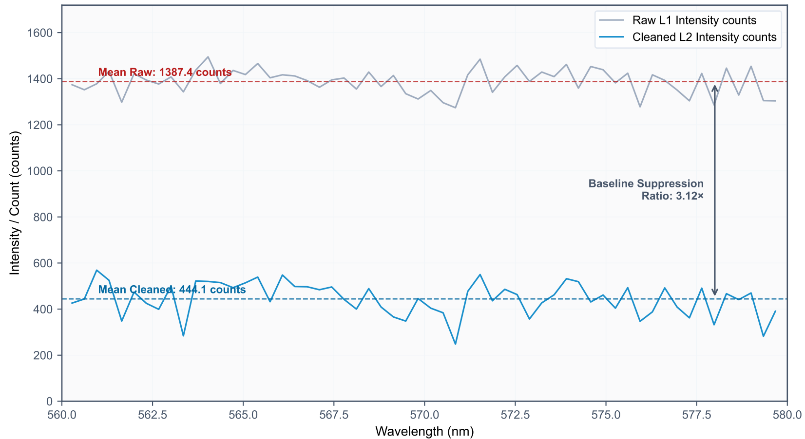
Figure F3: Pre- vs. Post-Subtraction Spectrum Overlay (560–580 nm Window)
