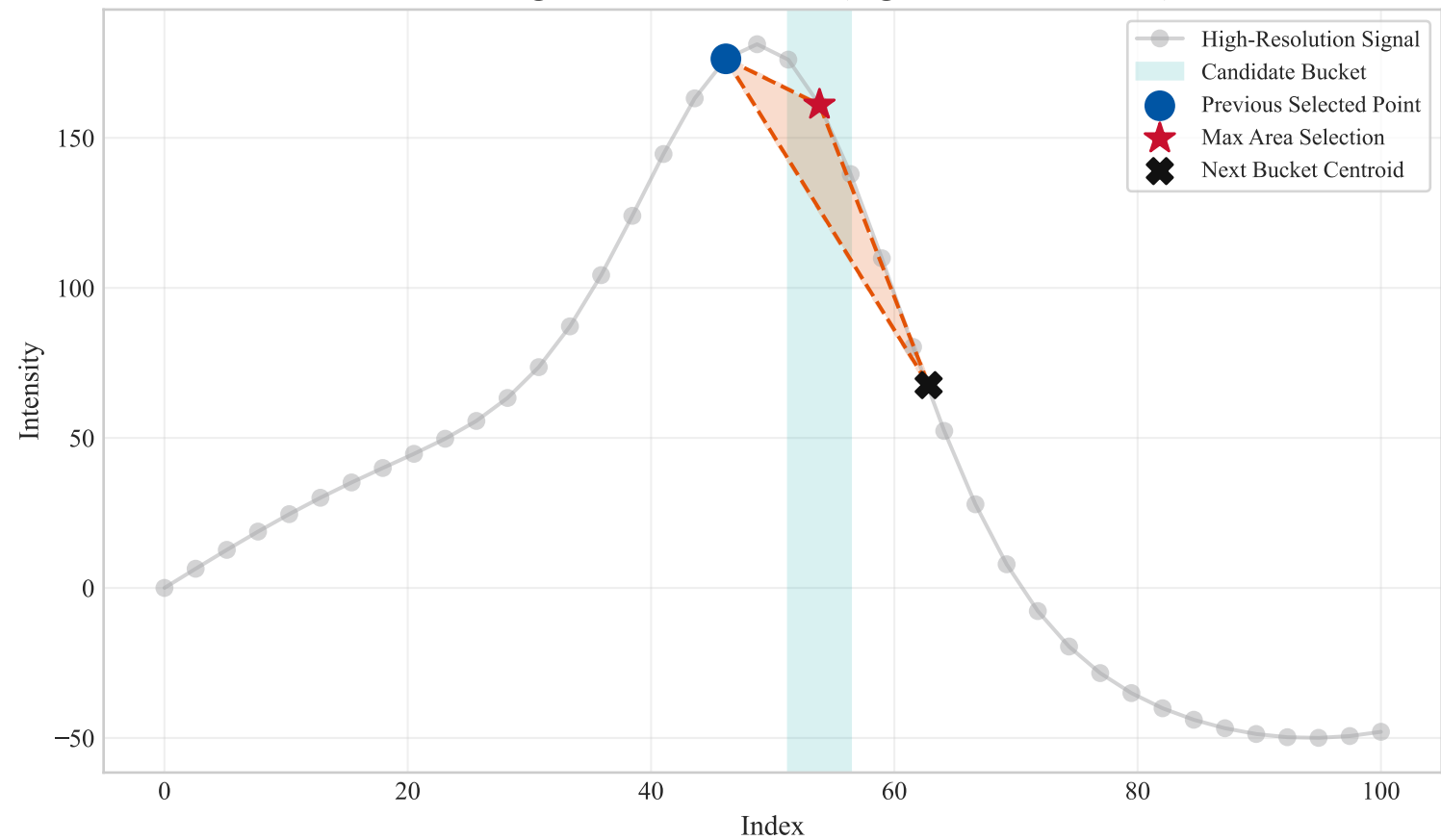
LTTB Triangle Area Maximization (Algorithmic Illustration)
