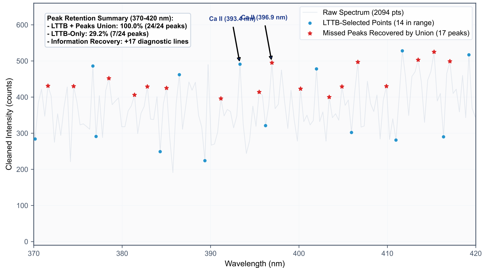
Figure F5: LTTB+Peaks vs LTTB-Only Peak Retention Comparison (Zoomed View)
