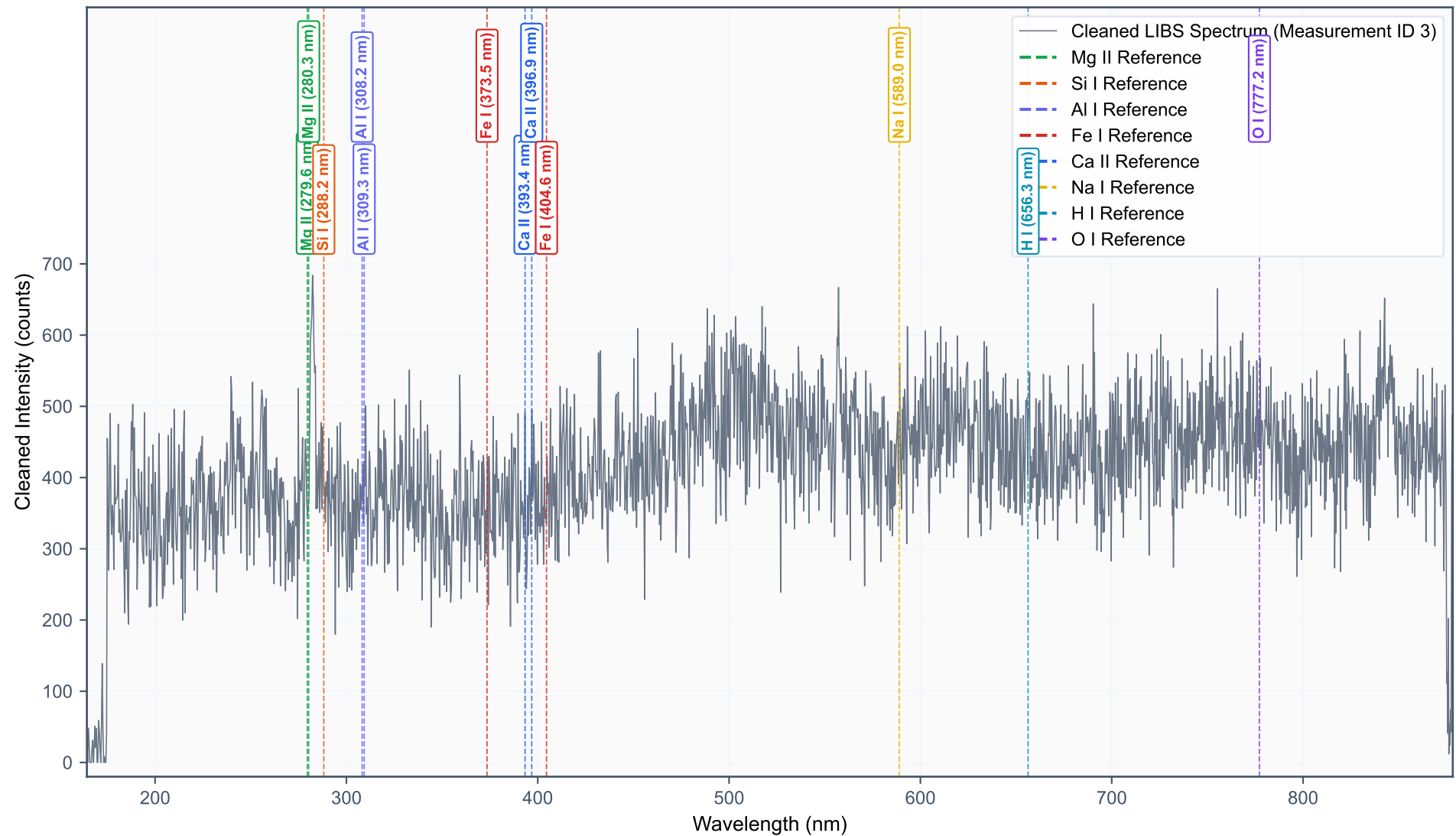
Figure F7: NIST Reference Line Overlays on Cleaned LIBS Spectrum
