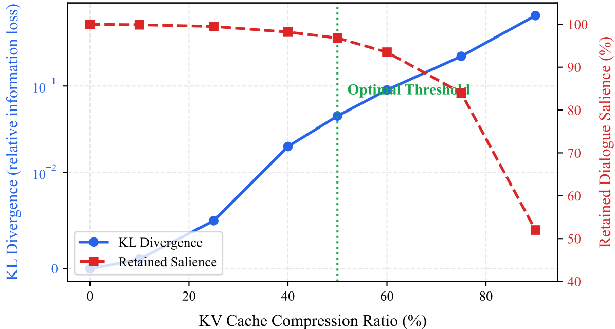
KV Cache Compression Information-Saliency Trade-off
