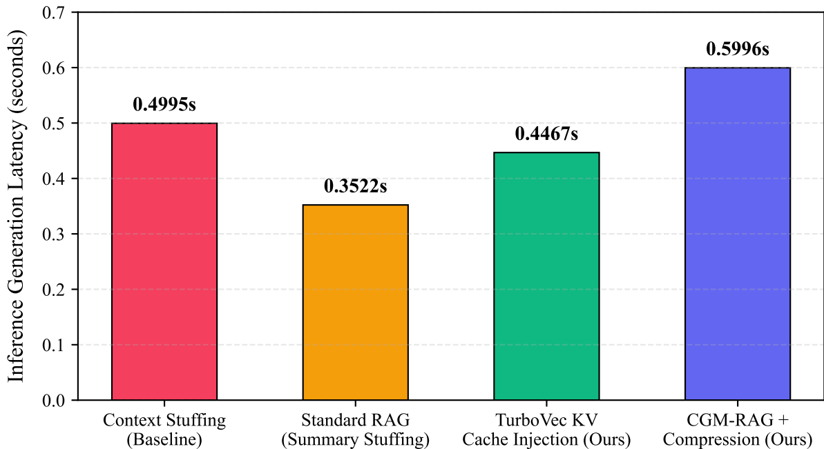
Dialogue Turn Inference Latency Comparison
