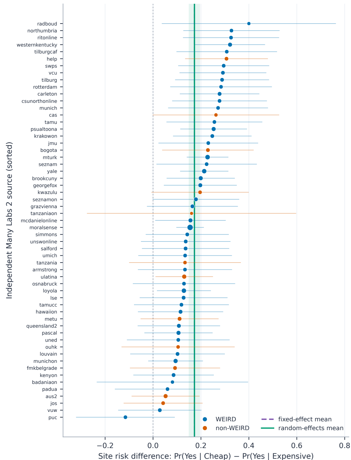
A Cross-site causal-effect variation
