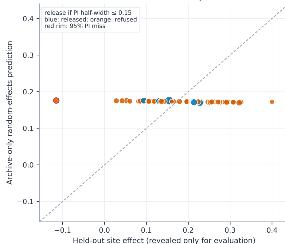
C Selective prediction frontier
