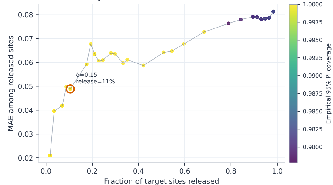
C Selective prediction frontier
