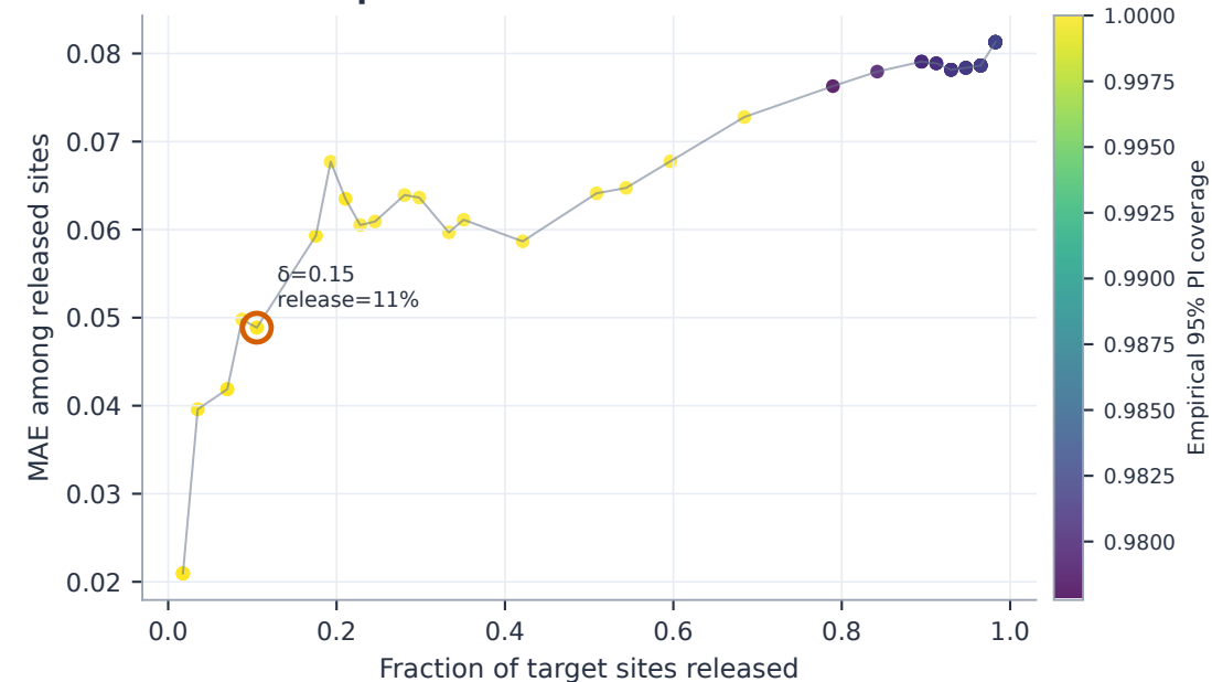
C Selective prediction frontier
