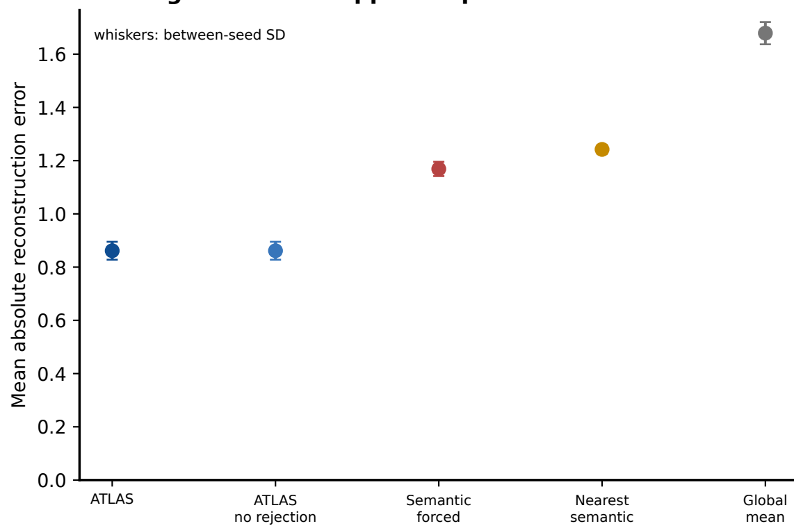
B Design-enriched support improves reconstruction
