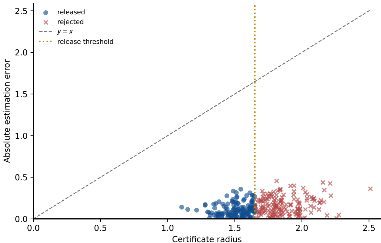
Certificate radius versus realized error
