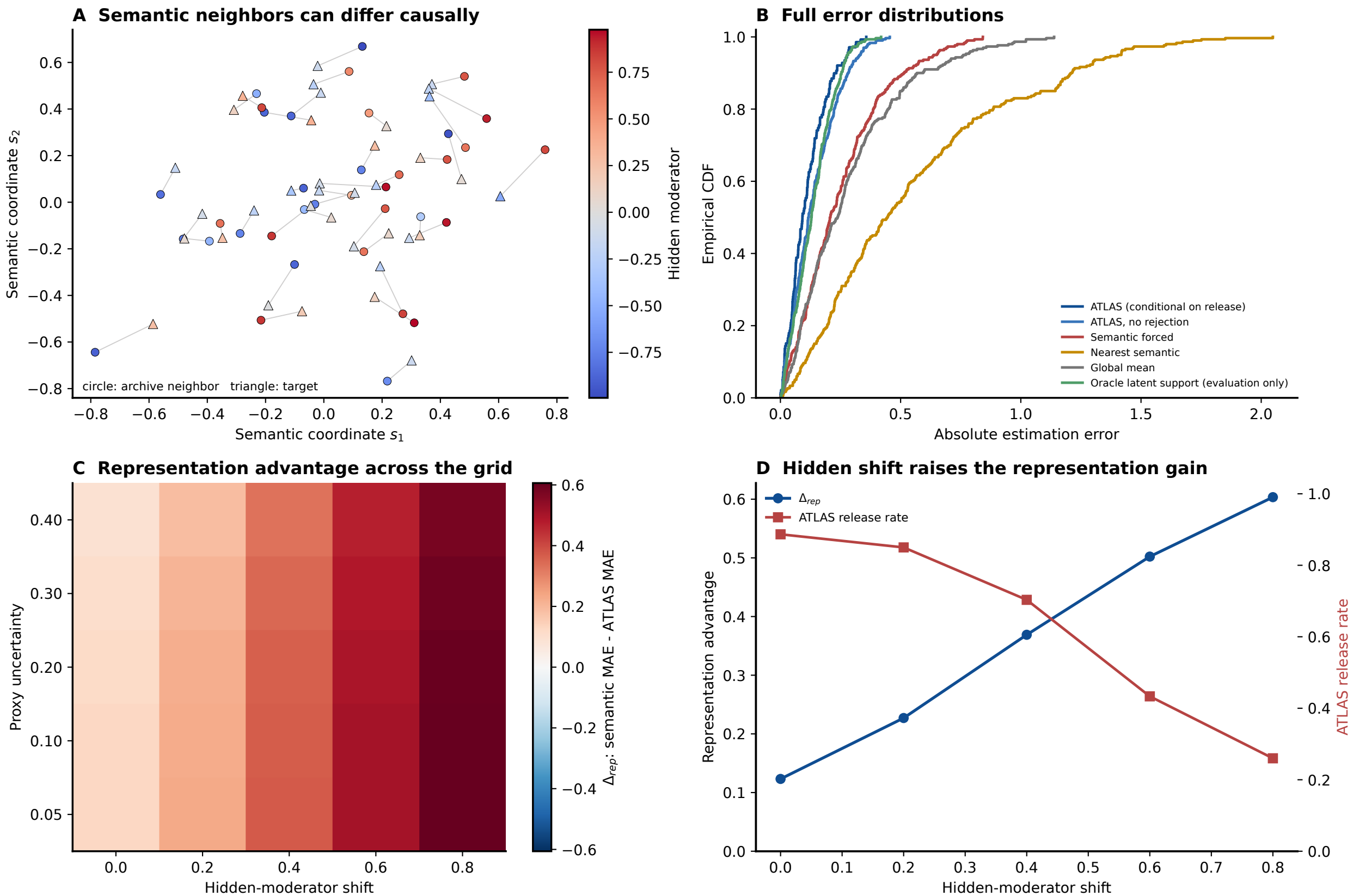
Figure 2. Synthetic validation of causal composability
