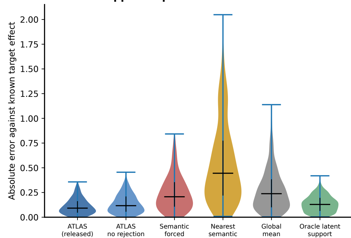
B Causal support improves reconstruction
