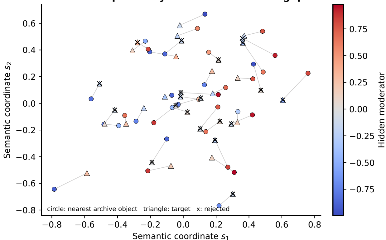
C Targeted bridges shrink the unidentified region fastest
