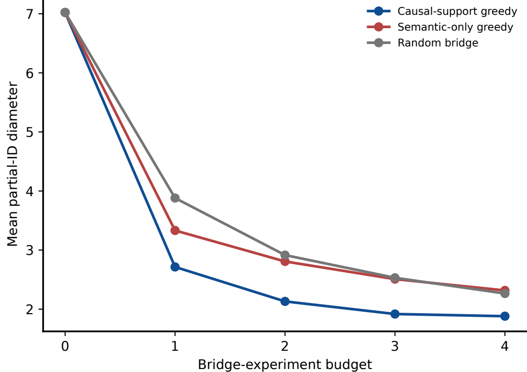
C Targeted bridges shrink the unidentified region fastest
