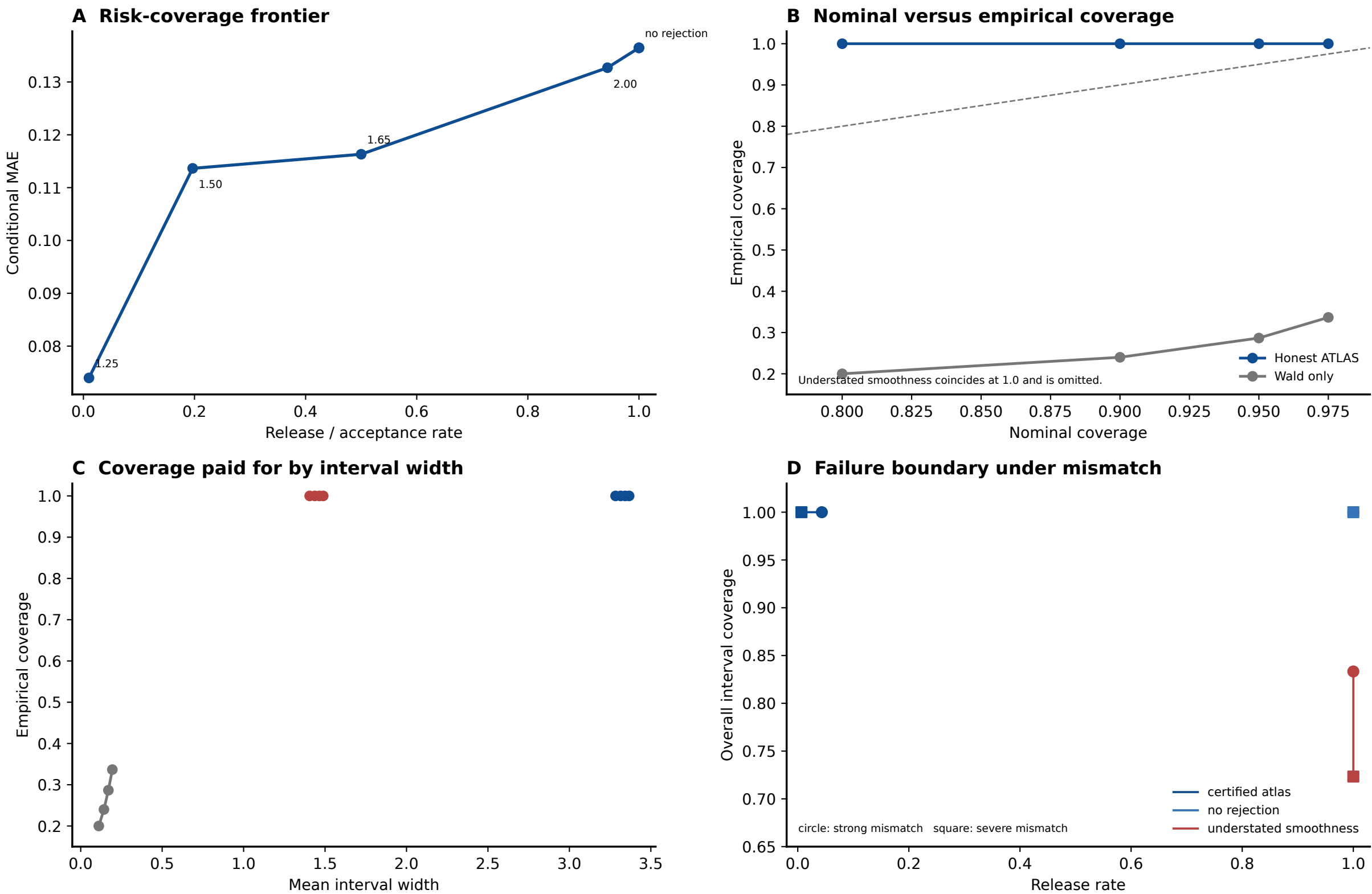
Figure 3. Selective prediction and honest uncertainty
