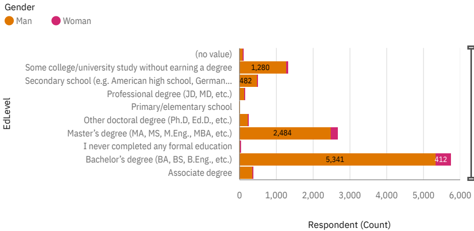
Respondent Education Level Split by Gender
