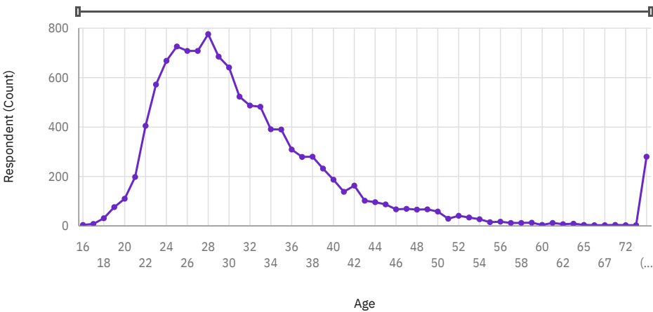
Respondent Age Curve
