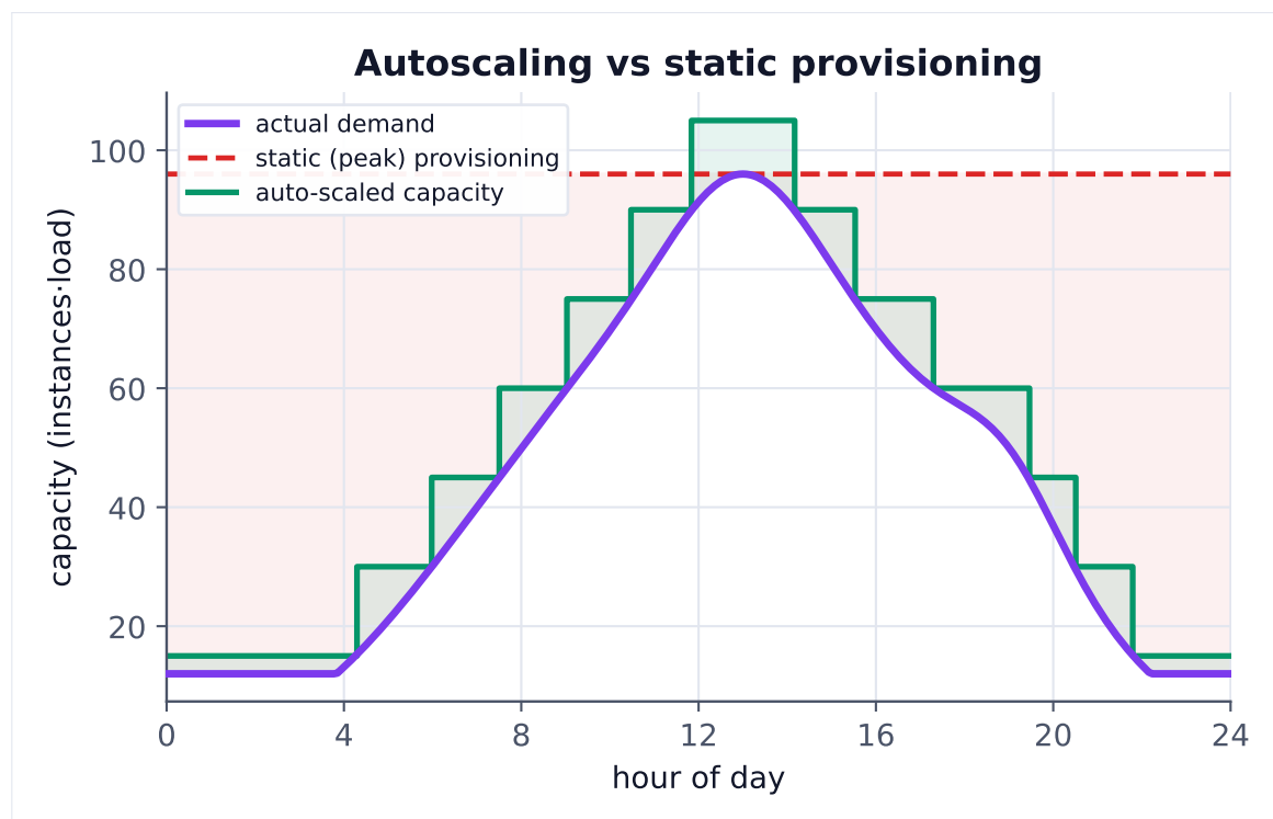
Figure 3. Static peak provisioning wastes capacity (red area) most of the day. Autoscaling tracks demand in steps, trading a little headroom for large cost savings.
