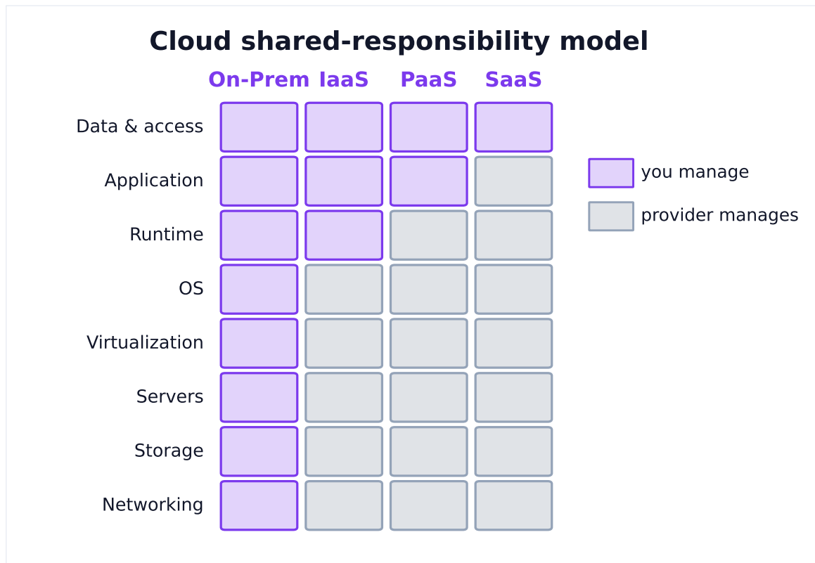
Figure 2. Moving from IaaS to SaaS hands more of the stack to the provider. Knowing the boundary tells you what you must still secure, patch and scale yourself.
